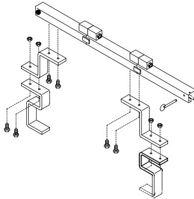
HOIST TOP RAIL PARTS WITH ELEVATING BRACKETS ILLUSTRATION 1-6
